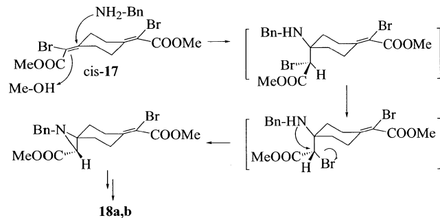
Figure 1. Proposed detailed mechanism for the anti protonation and spiroaziridination following the hetero-Michael addition reaction.
